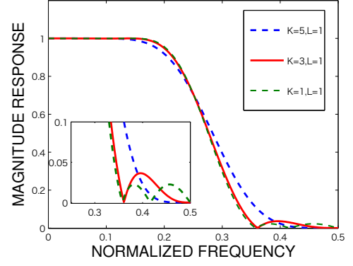
Fig. 2. Magnitude responses of scaling lowpass filters H_i(z) .
