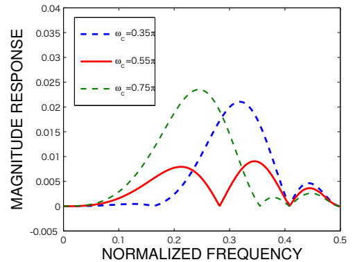
Fig. 4. Magnitude responses of E(\omega) .
