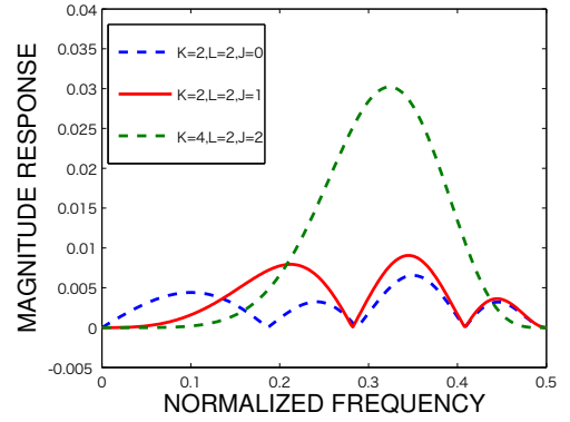
Fig. 3. Magnitude responses of E(\omega) .
