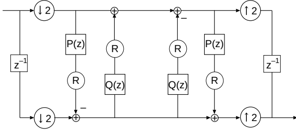
Fig. 1. Lifting scheme
